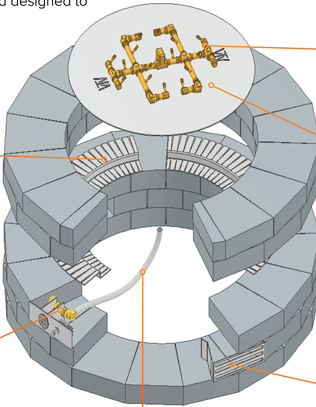
CROSSFIRE® Brass Burner (CFB180)
